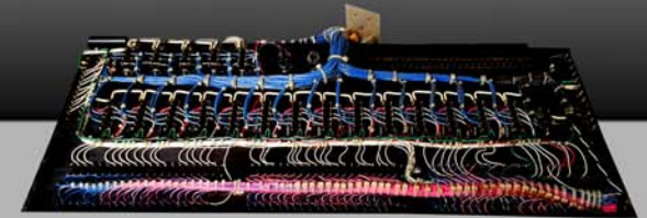
Signal Switching Harness Assembly
